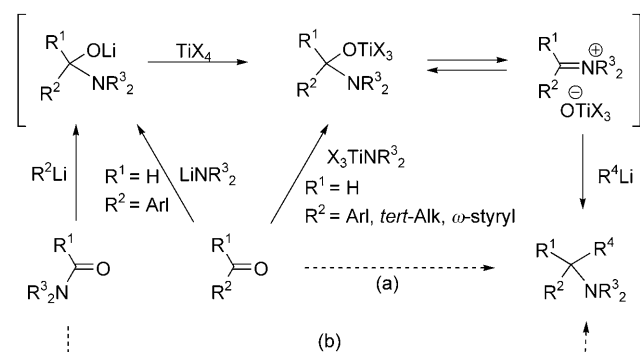
Scheme 4. a) Alkylation of aromatic (or other non-enolizable) aldehydes [5–7,27–31,33] and b) geminal disubstitution of amide oxygens [7] via \alpha -amino–Li and –Ti alkoxides; when R 4 Li is a Li enolate, Mannich bases are formed. [33b] For examples see Table 2.
