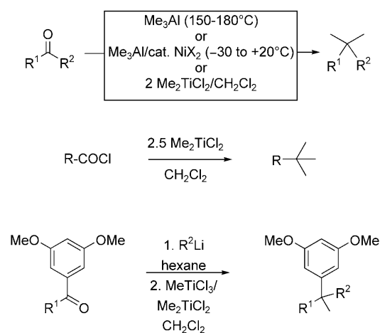
Scheme 5. Di- and trimethylations and alkylative methylation of ketones and acid chlorides with Me 3 Al [42] and Me–Ti reagents. For reviews on the Ti reagents see Refs. [30, 31]; for examples see Table 3.
