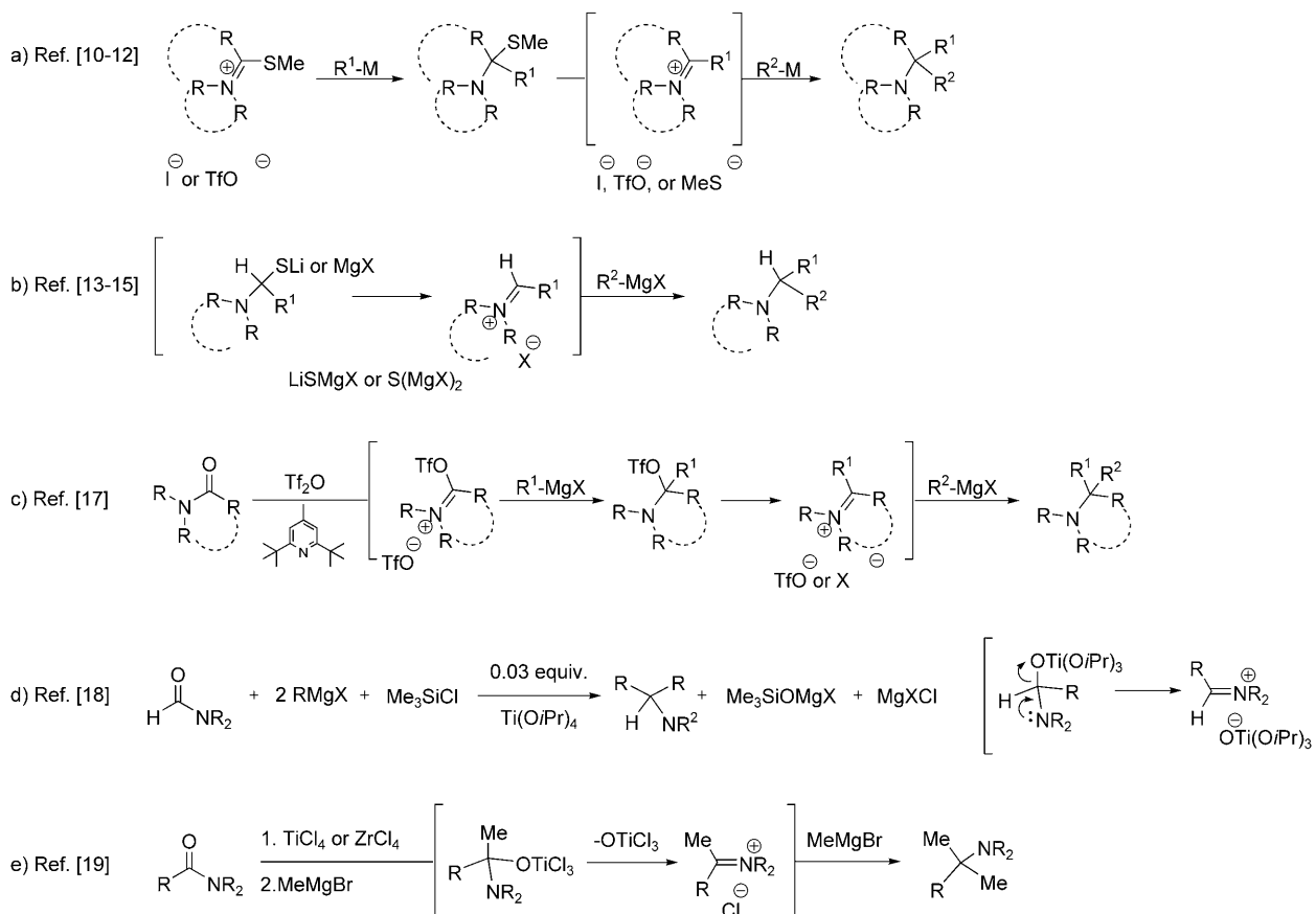
Scheme 3. Procedures for the geminal disubstitution of amide carbonyl oxygens with formation of tertiary sec - and tert -alkylamines and proposed reactive intermediates. [10-15,17-19] The thioamide precursors for reactions (a) and (b) are prepared from amides and lactams, respectively, with the Lawesson reagent. For examples see Table 1.
