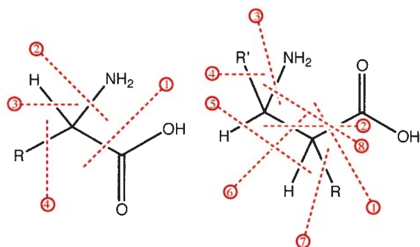
Fig. 2 Retrosynthetic analysis of an α- and a β-amino acid. The numbers ①–⑧ indicate the bond(s) made in the corresponding synthesis. For literature on α- and β-amino acid syntheses, see textbooks, monographs and a book (ref. 9), which has appeared recently.
