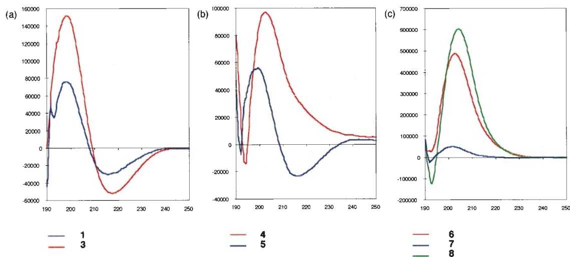
Fig. 5 Circular dichroism (CD) spectra of \beta -peptides 1,3–8 in MeOH (0.2 mm). The typical CD pattern assigned to a left-handed 3_1 helix [cf. Figs. 1(b) and 6(a)] is shown in (a) and the blue curve in (b). The characteristic CD pattern of a secondary structure which is, as yet, unassigned is shown in (c) and the red curve in (b). The most intensive Cotton effects were measured with disubstituted \beta -amino acid moieties [ 3 , red in (a)], with a ( \beta^2 ) 3 ( \beta^3 ) 3 (protected) sequence [ 4 , red in (b)] and with the protected ( \beta^2, \beta^3 ) 6 dodecapeptide [ 8 , green in (c)].
