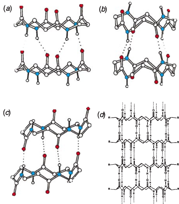
Fig. 11 Arrangement of the cyclo- \beta -tetrapeptides (a) 12, (b) 13 and (c) 14 as found in the solid state (cf. Fig. 8). All hydrogen-bonded rings are 14-membered with (7 + 7) and (8 + 6) combinations of the participating fragments. Me substituents and hydrogen atoms bound to carbon are omitted for clarity. For comparison, the stacking of a cyclo- \alpha -octapeptide with alternating configuration of the residues is shown in (d). [Taken with permission from refs. 28 and 35(c).]
