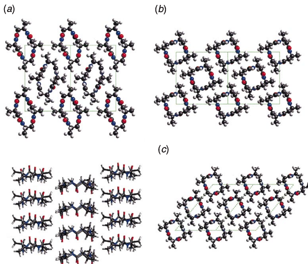
Fig. 8 Tubular stacking of cyclo- \beta -tetrapeptides in the solid state (from powder diffraction data). (a) 12 [(S,S,S,S); top view (above), side view (below)]; (b) 13 [(R,S,R,S)], top view; (c) 14 [(R,R,S,S)], top view. In 12 , the ring adopts a rhomboidal shape, in 13 , a square and in 14 , a rectangular shape. All four C=O and N–H bonds are unidirectional in (a), two C=O and two N–H bonds point up and down on opposite faces in (b) and on adjacent faces in (c). (Taken with permission from ref. 28.)
