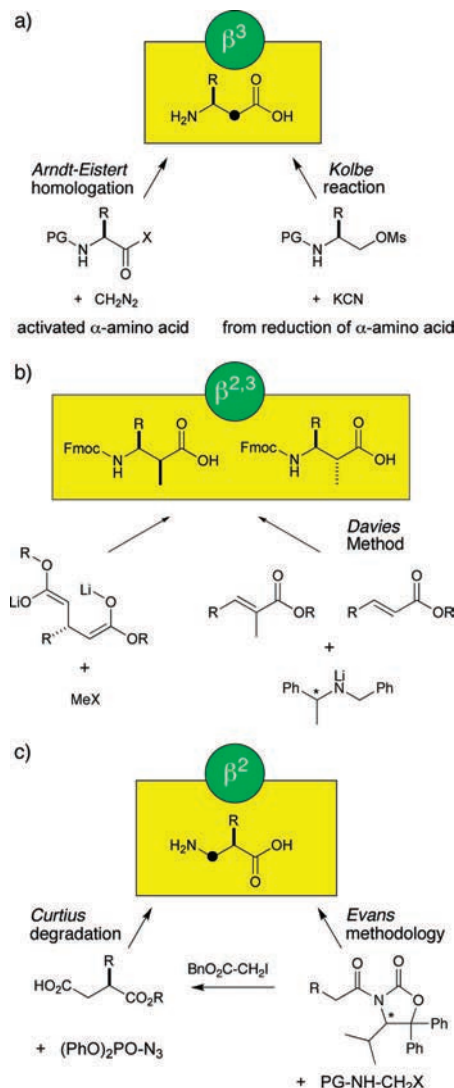
FIGURE 2. Generally applicable methods used by us for the preparation of the various types of \beta -amino acids with the 21 proteinogenic side chains R: (a) stereospecific classical homologation of \alpha -amino acids (H-Xaa-OH) by insertion or addition of a one-carbon moiety to give \beta^3 -amino acids (H- \beta^3 hXaa-OH); (b) \alpha -methylation of a \beta -amino acid derivative or overall enantioselective Michael addition of \text{NH}_2/\text{H} or \text{NH}_2/\text{CH}_3 to an acrylate ester for preparation of \beta^{2,3} -amino acids; (c) overall enantioselective aminomethylation of a “des-amino” acid, directly or through a succinic acid half-ester, to provide \beta^2 -amino acids (H- \beta^2 hXaa-OH).
